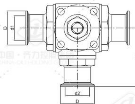
1"-4"Non-Encapsulated and ISO mounting pad. Flange connection size please refer to the standard ISO5211
