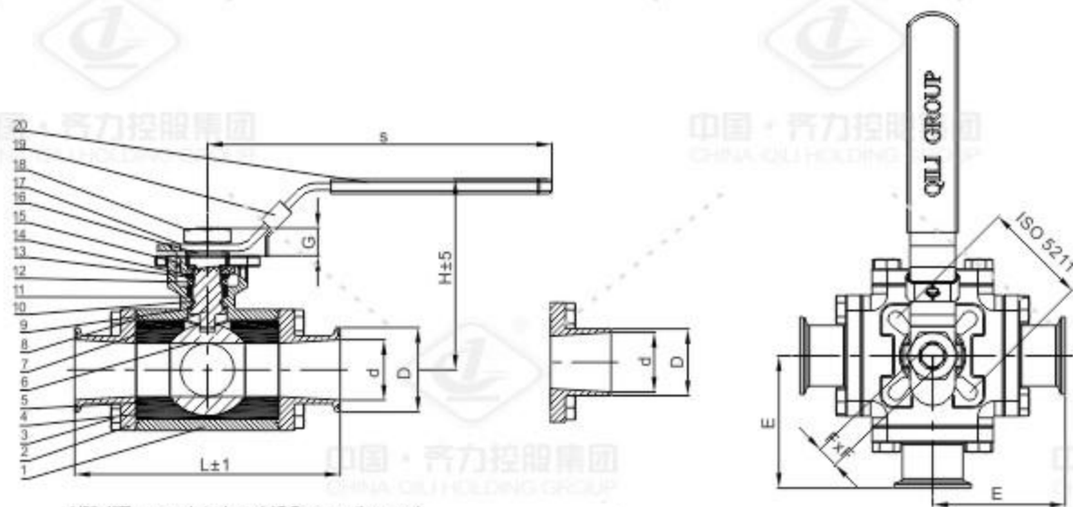
1/2"-4"Encapsulated and ISO mounting pad. Mounting pad connection size please refer to the standard ISO5211
