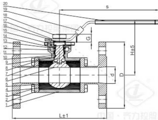
1/2"-4"Encapsulated and ISO mounting pad. Flange connection size please refer to the standard ISO5211
