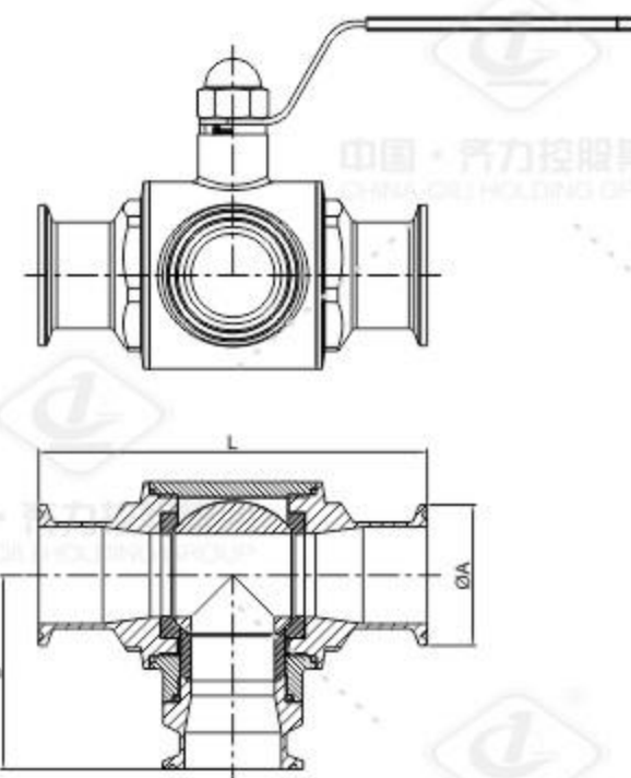
手动缩径三通球阀 Manual reducing three-way ball valve
