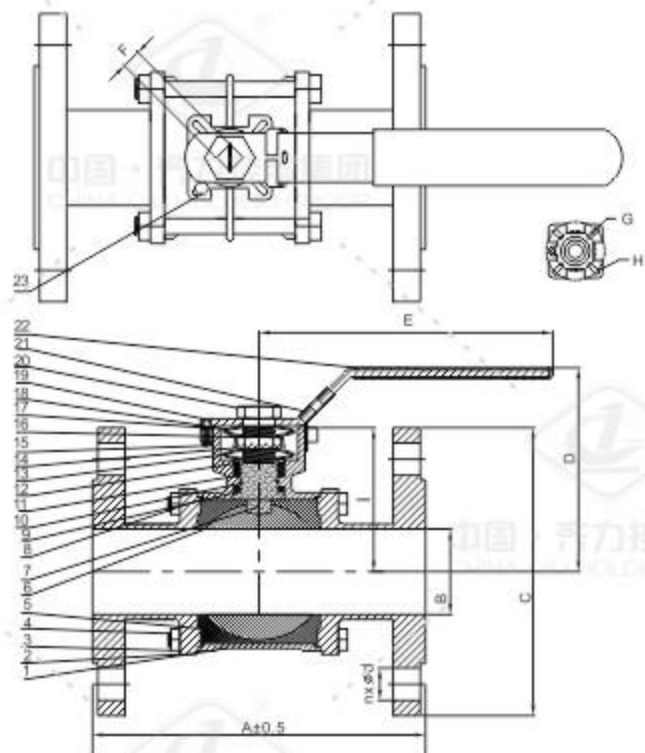
1/2"-6" Encapsulated and ISO mounting pad.
