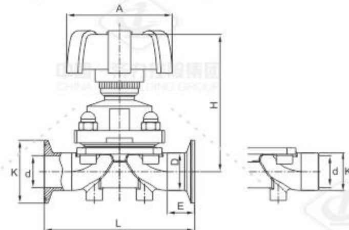
New generation diaphragm valve
